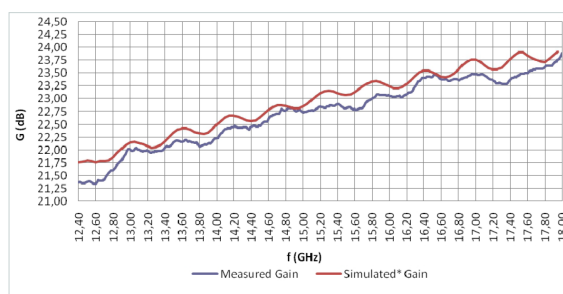
ASY-SGH-124 Gain
