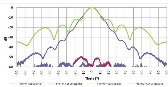
ASY-SGH-124 Radiation Patterns f=15.20 GHz
