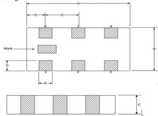
Layout Drawing
