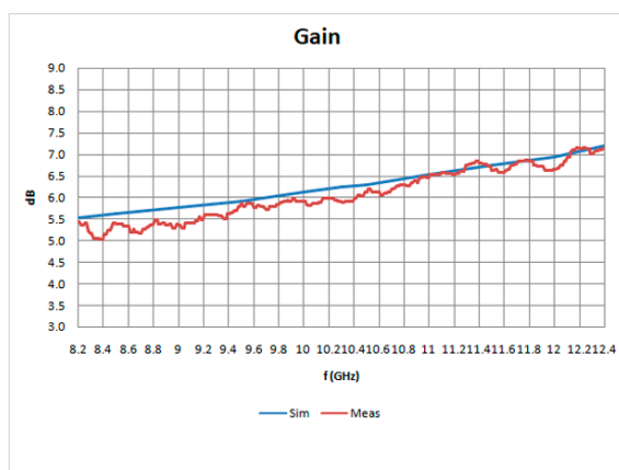
Simulated vs. measured gain over frequency
