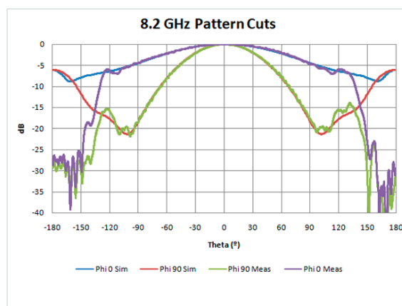
Simulated vs measured radiation pattern at 8.2GHz
