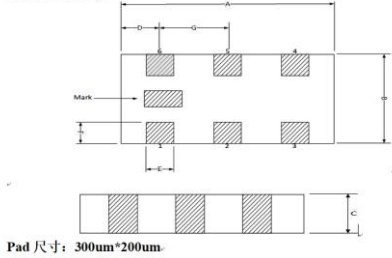
Layout Drawing
